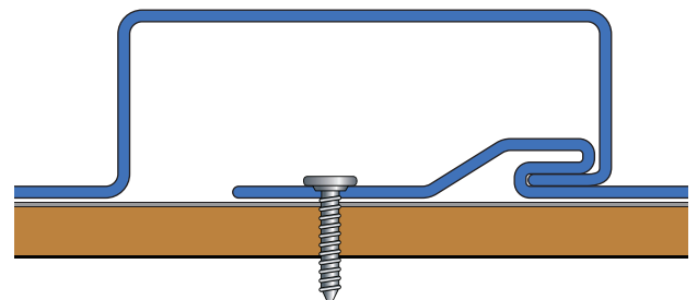
Panel overlap detail
