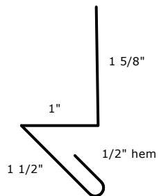
BASE ANGLE STOP
