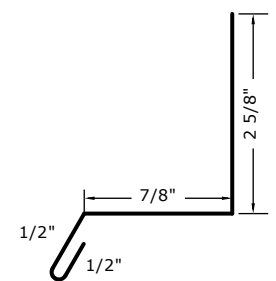
BASE DRIP ANGLE
