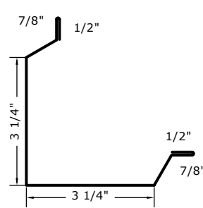
GAMBREL TRIM
