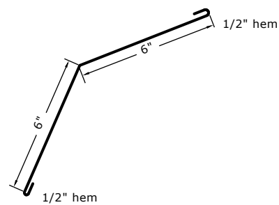
GAMBREL TRIM
