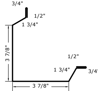
GAMBREL TRIM
