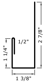
J CHANNEL
