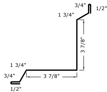
TRANSITION TRIM
