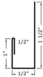
J CHANNEL
