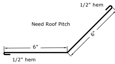
TRANSITION TRIM
