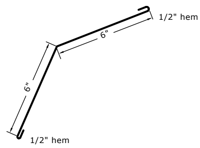
GAMBREL TRIM
