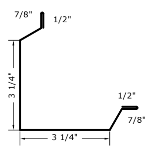
GAMBREL TRIM
