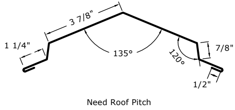
STEPPED RIDGE
